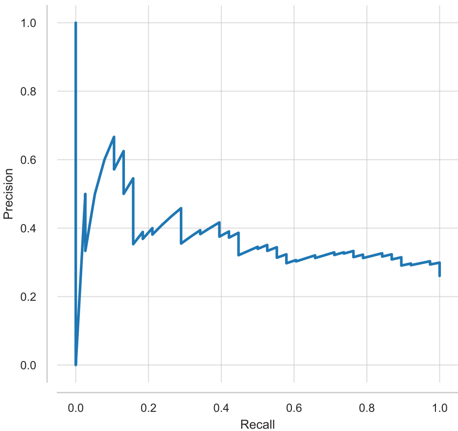
Precision-Recall Curve - HGB
